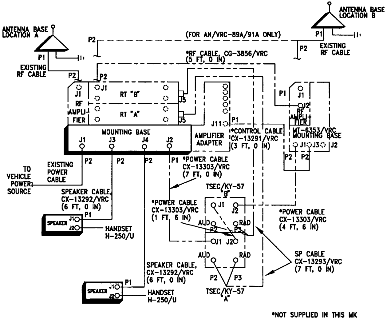
Figure 5-7(2). Cable Diagram: For AN/VR-89/91/92
